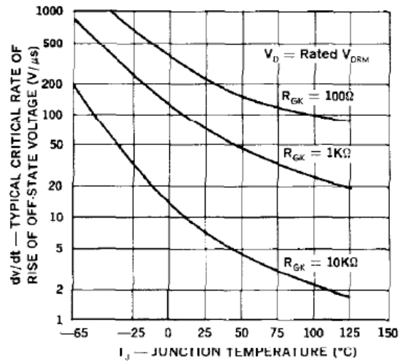
dv/dt vs. Junction Temp.
