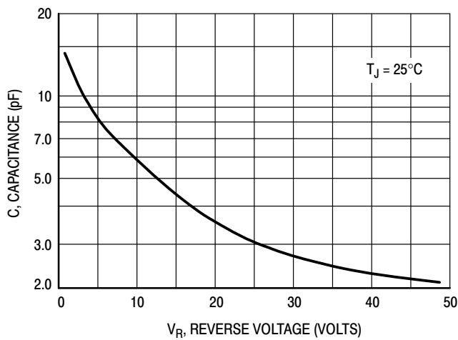
Figure 10. Typical Capacitance
