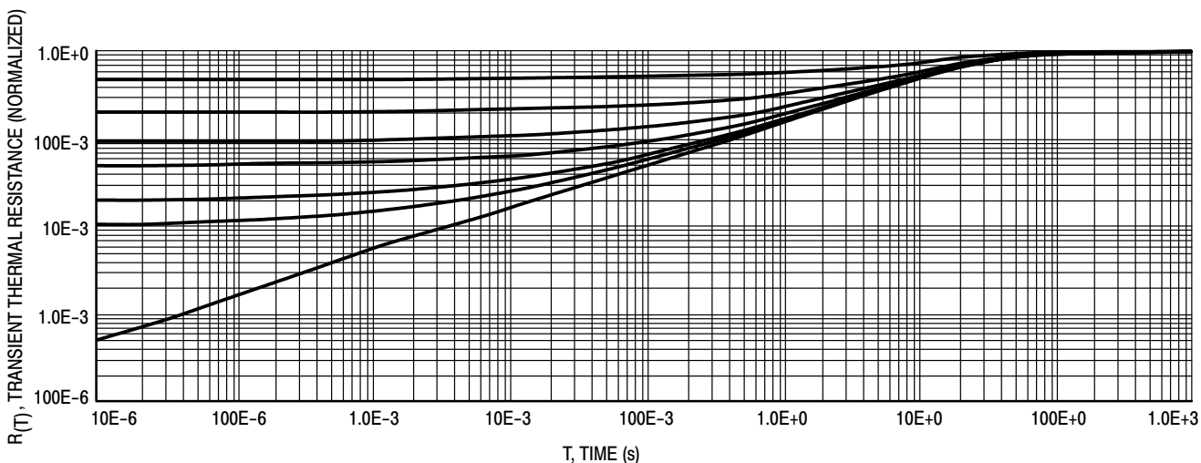
Figure 7. Thermal Response
