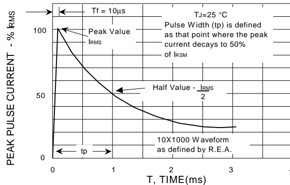
FIG.3 - PULSE WAVEFORM
