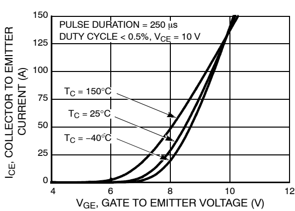
Figure 1. TRANSFER CHARACTERISTICS
