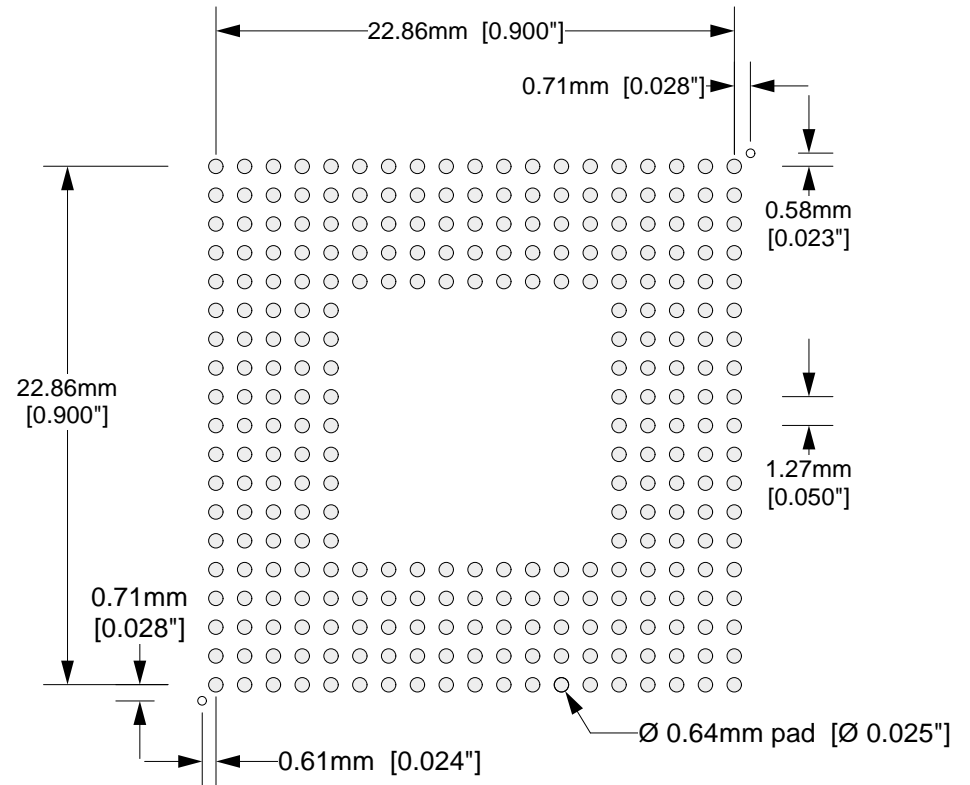
Top View: Recommended PCB Layout Scale: 3:1
