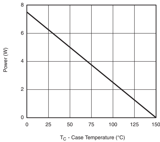
Power, Junction-to-Case
