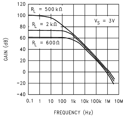
Figure 5-19. Open Loop Frequency Response
