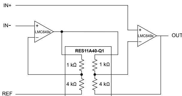
Two-Op-Amp Instrumentation Amplifier Using the RES11A-Q1
