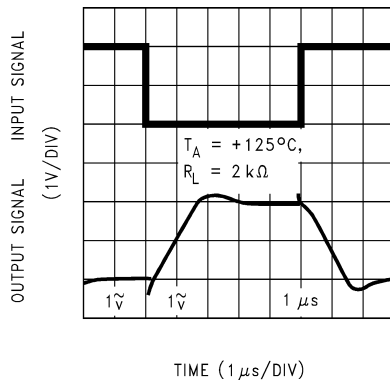
Figure 5-31. Inverting Large Signal Pulse Response
