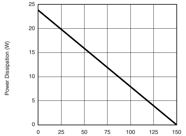
Power Derating
