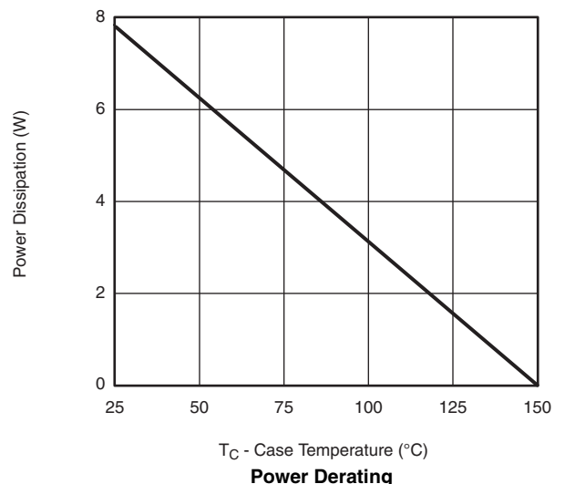
Power Derating
