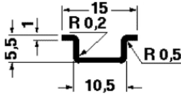
Dimensioned drawing
