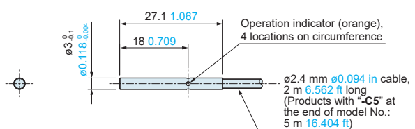
GX-305S-□ Sensor
