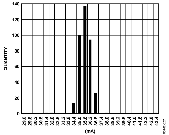
Figure 27. Fast Mode Power Supply Current Distribution at 25°C/3.3 V
