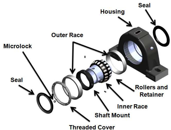
Figure 1) Exploded View of 2000 Series Bearing
