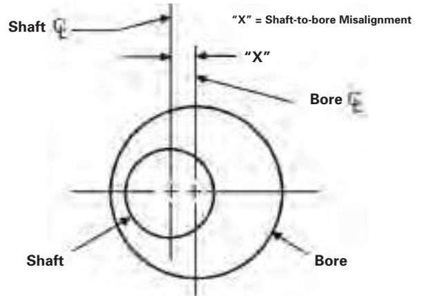
Figure 5: Shaft-to-bore Misalignment
