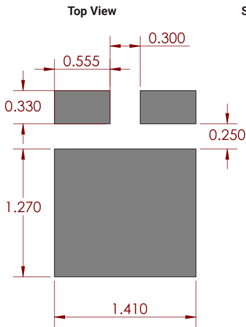
Recommended Solder Pad (Solder Mask Pattern)
