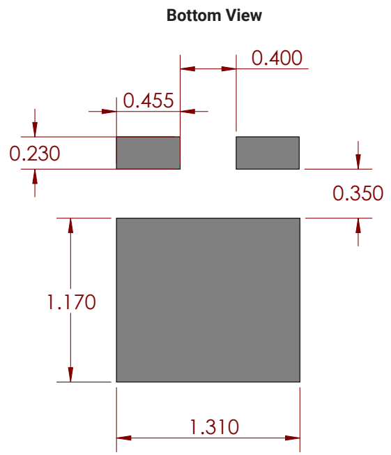
Recommended Stencil Openings
