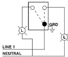
Wiring Diagram Single-Pole, Double Throw (SPDT) Center OFF
