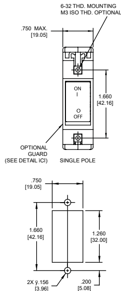
Panel Mounting Detail Mounting Detail Tolerance: \pm .005 [.13] unless noted
