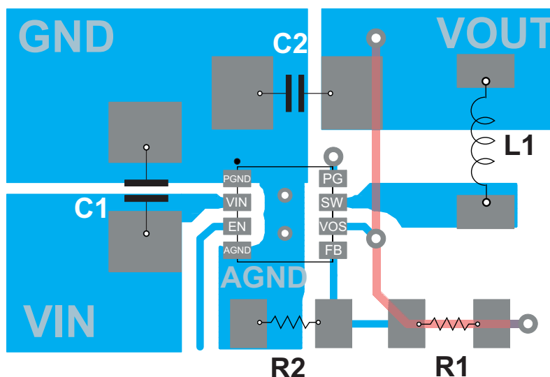
Figure 42. Layout Example
