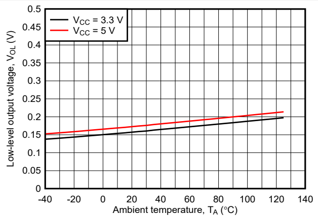
Figure 7-6. Low-Level Output Voltage vs Ambient Temperature
