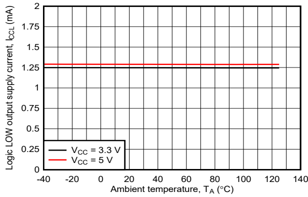
Figure 7-15. Logic LOW Output Supply Current vs Ambient Temperature
