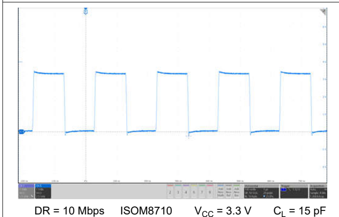
Figure 10-4. Typical Output Waveform at I_F = 3 mA
