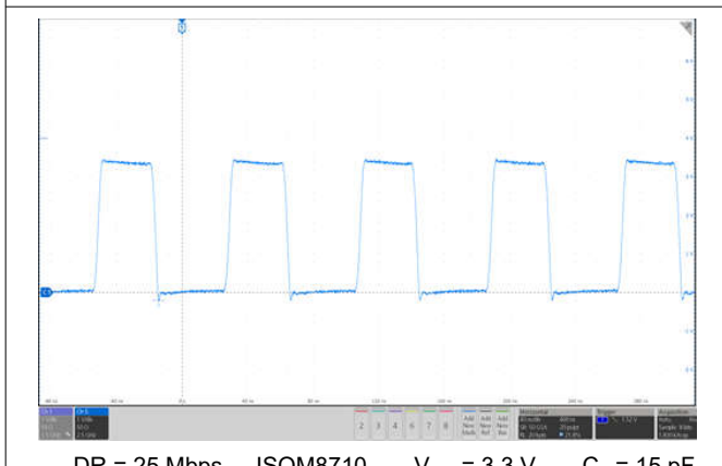
Figure 10-6. Typical Output Waveform at I_F = 6 mA
