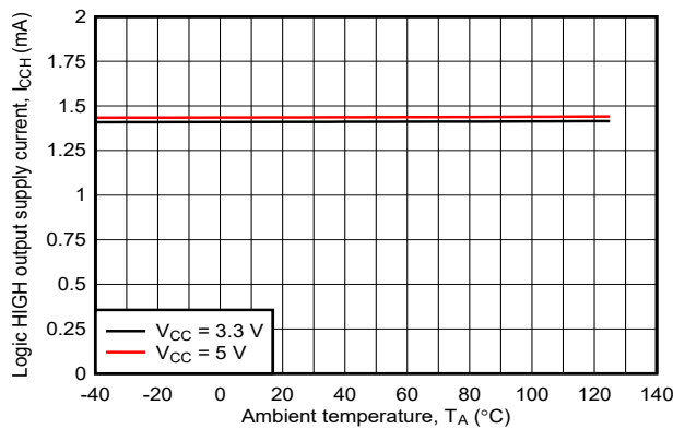
Figure 7-17. Logic HIGH Output Supply Current vs Ambient Temperature
