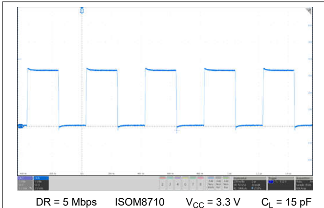
Figure 10-2. Typical Output Waveform at I_F = 2 mA
