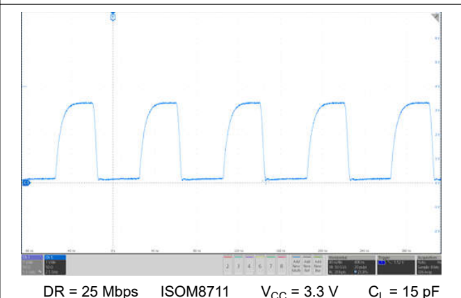
Figure 10-7. Typical Output Waveform at I_F = 6 mA
