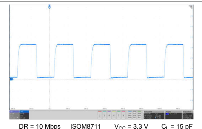
Figure 10-5. Typical Output Waveform at I_F = 3 mA
