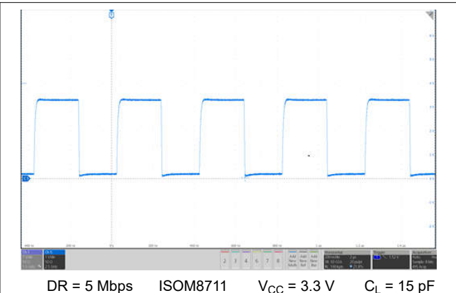
Figure 10-3. Typical Output Waveform at I_F = 2 mA
