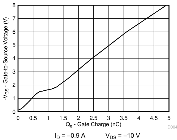
Figure 5-4. Gate Charge
