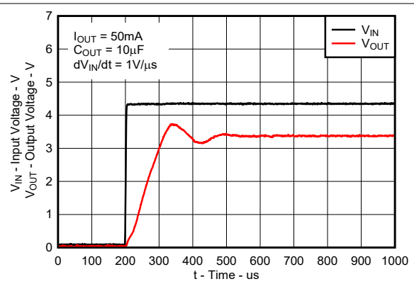
Figure 5-26. Fast Power-Up (Legacy Chip)
