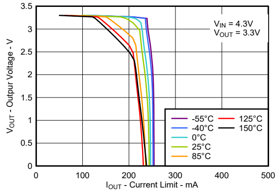
Figure 5-20. Output Voltage vs Current Limit (New Chip)
