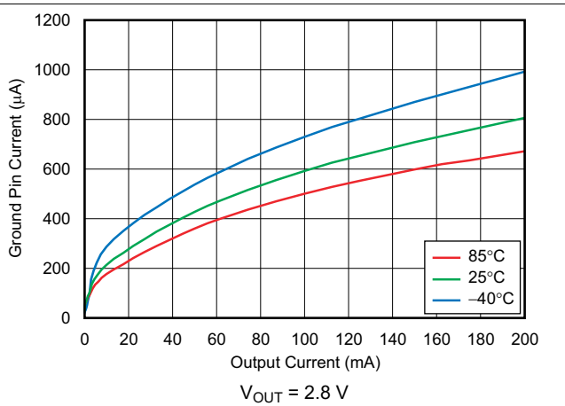
Figure 6-24. Ground Pin Current vs Output Current
