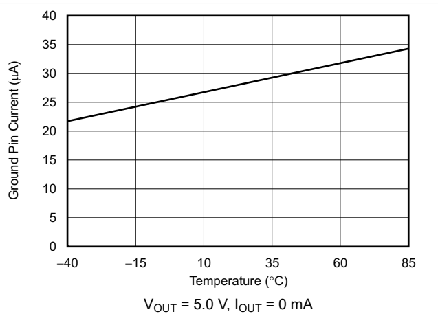
Figure 6-22. Ground Pin Current vs Temperature
