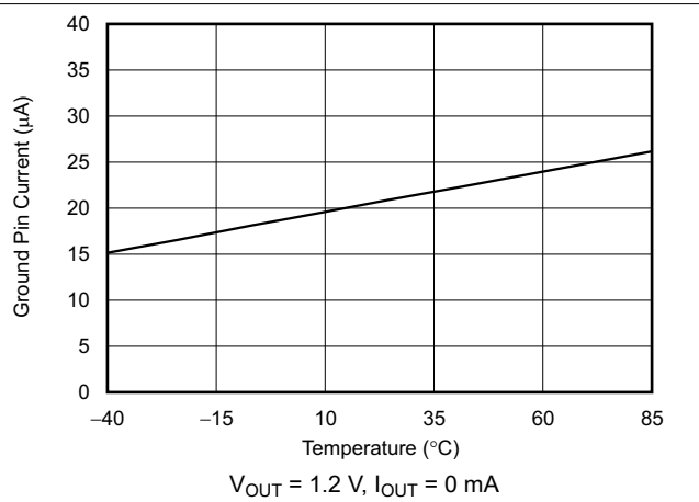
Figure 6-20. Ground Pin Current vs Temperature
