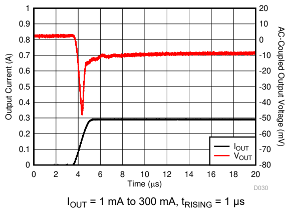
Figure 6-51. Load Transient
