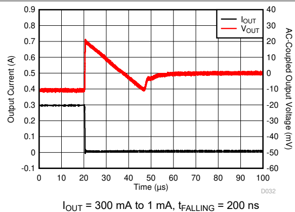
Figure 6-54. Load Transient
