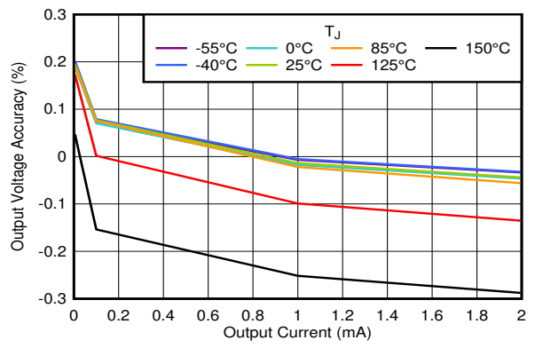
Figure 6-18. Output Voltage Accuracy vs I_{OUT}
