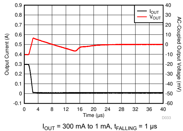
Figure 6-52. Load Transient
