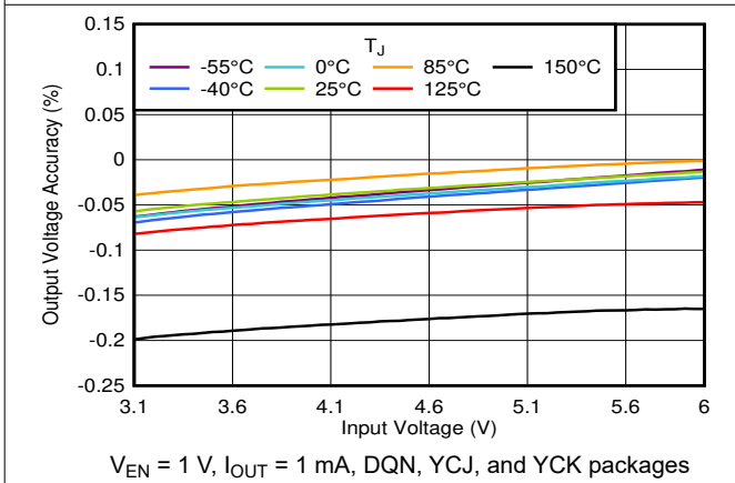
Figure 6-21. Output Voltage Accuracy vs V_{IN}
