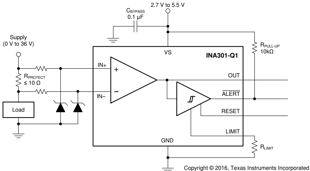
Figure 8-3. Transient Protection
