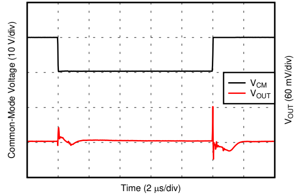
Figure 6-26. Common-Mode Voltage Transient Response
