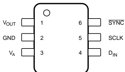
6-Pin (SOT-23) Top View
