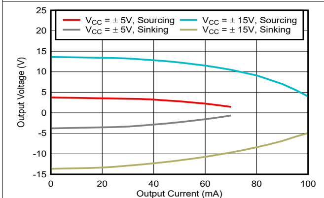
Figure 6-29. Output Swing vs Load Current
