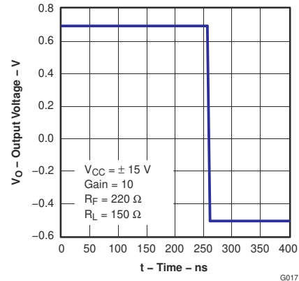
Figure 6-46. 1-V Step Response
