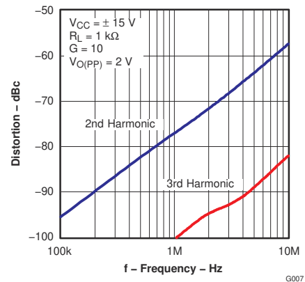
Figure 6-36. Distortion vs Frequency
