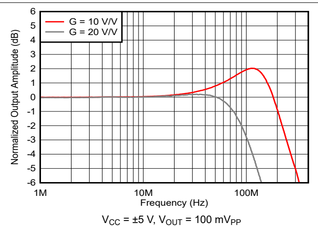
Figure 6-4. Frequency Response vs Gain
