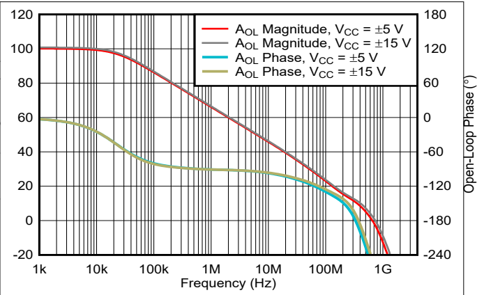
Figure 6-8. Open-loop Gain and Phase Response
