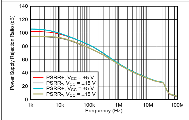
Figure 6-9. Power-Supply Rejection Ratio vs Frequency
