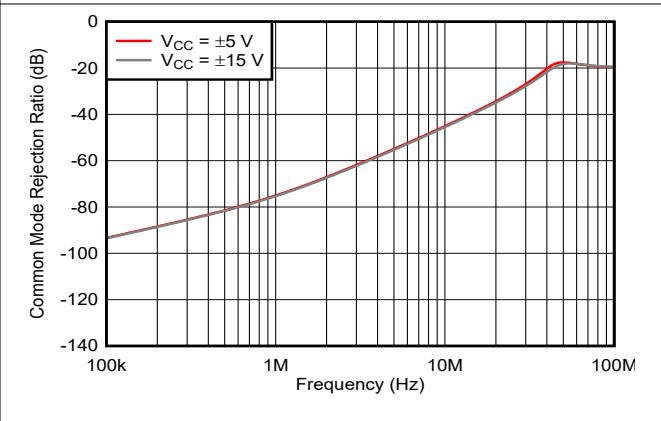
Figure 6-10. Common-Mode Rejection Ratio vs Frequency
