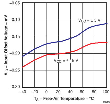
Figure 6-48. Input Offset Voltage vs Free-air Temperature
