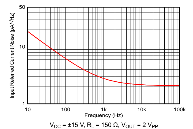
Figure 6-12. Input-Referred Current Noise vs Frequency
