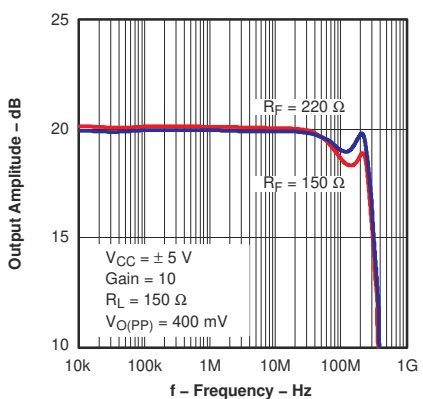
Figure 6-41. Output Amplitude vs Frequency
