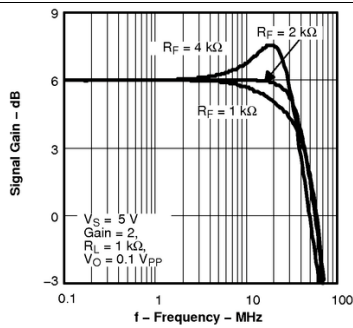
Figure 13. Frequency Response
