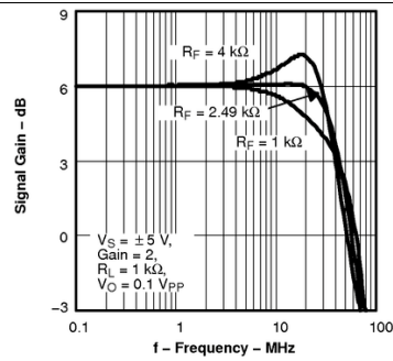
Figure 14. Frequency Response
