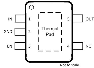
Figure 4-2. DYD Package (Preview), 5-Pin SOT-23 With Exposed Thermal Pad (Top View)
