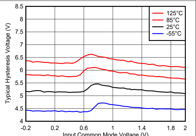
Figure 6-39. Hysteresis Voltage vs. Common Mode, 1.8V
