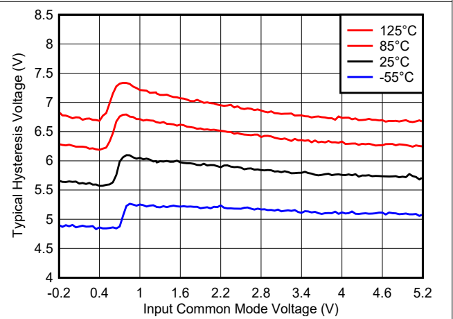
Figure 6-41. Hysteresis Voltage vs. Common Mode, 5V
