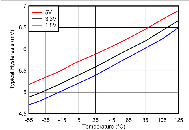
Figure 6-38. Hysteresis Voltage vs. Temperature
