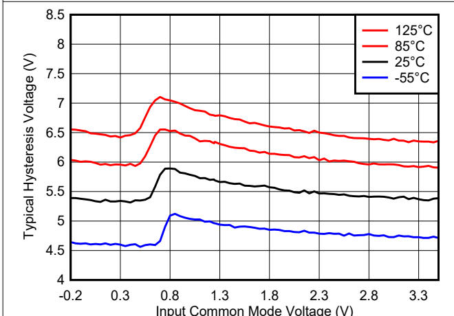
Figure 6-40. Hysteresis Voltage vs. Common Mode, 3.3V
