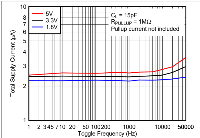
Figure 6-36. Supply Current vs. Toggle Frequency - Open Drain Output
