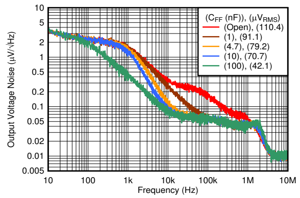
Figure 6-74. Output Noise vs Frequency and C_{FF}
