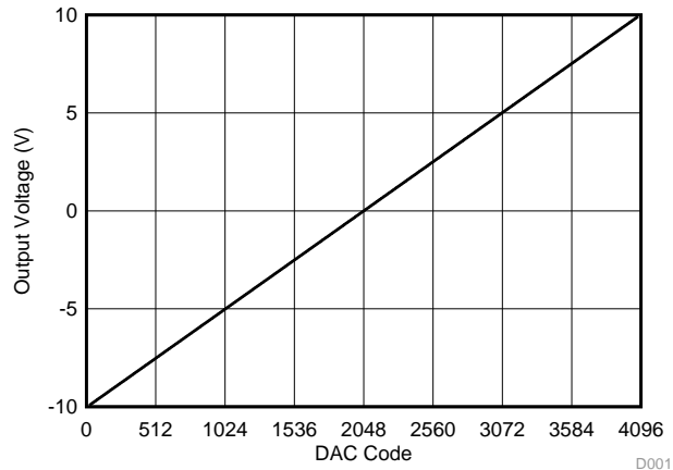
Figure 79. Bipolar Operation
