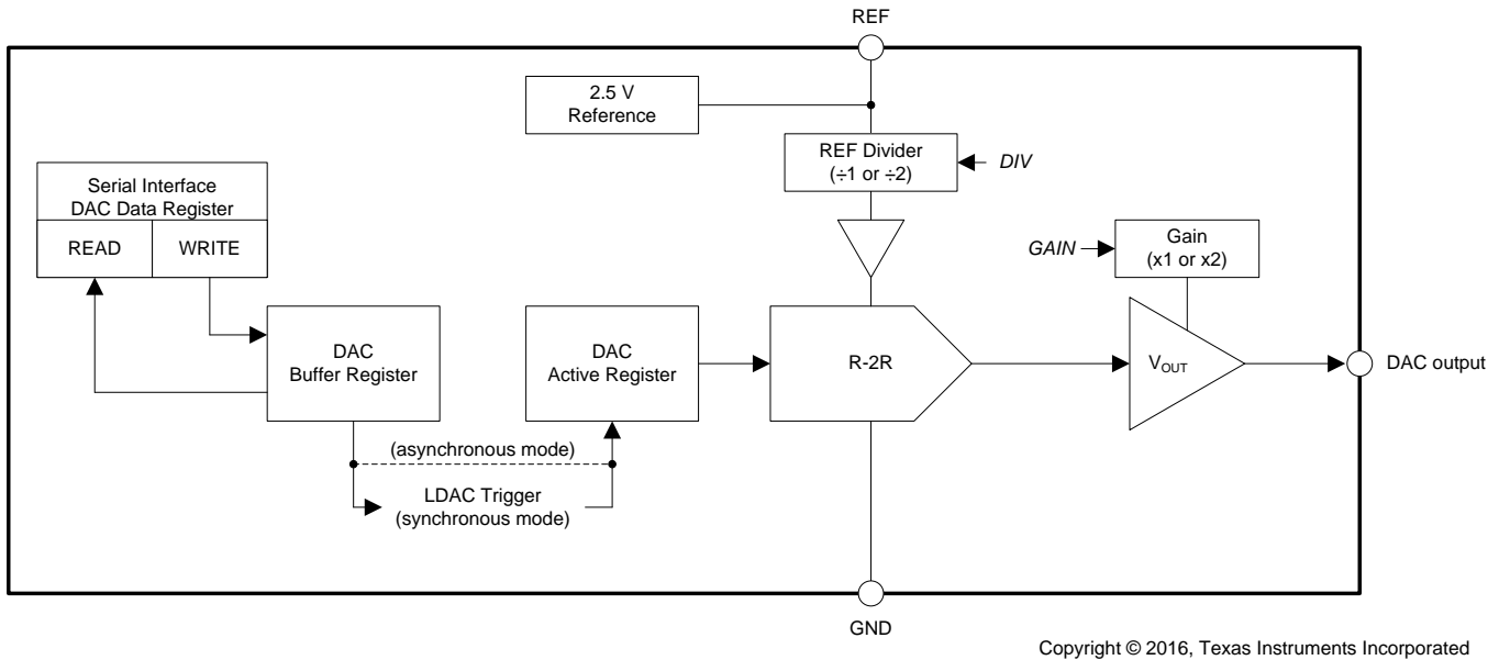
Figure 59. DACx0508 DAC Block Diagram
