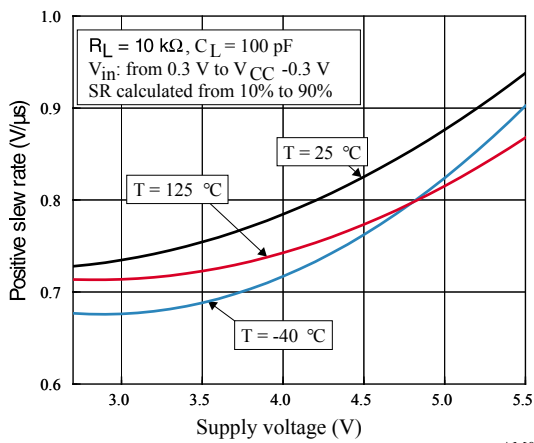
Figure 14. Positive slew rate vs. supply voltage
