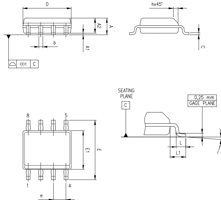
Figure 34. SO8 package outline
