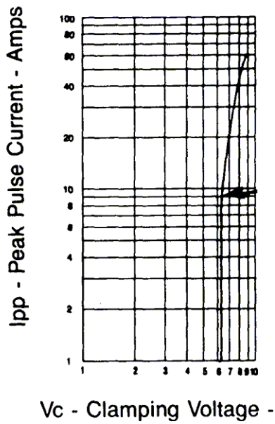
Figure 3-4. Typical Clamping Voltage ( V_C ) vs. Peak Pulse Current ( I_{PP} )
