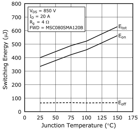
Figure 1-13. Switching Energy vs. Junction Temperature
