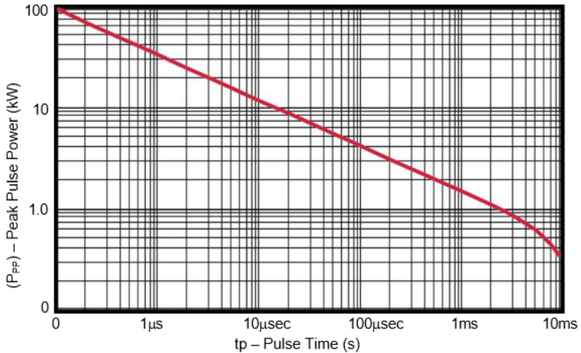
Figure 4-2. Pulse Waveform
