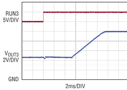
Soft Start-Up (Boost)
