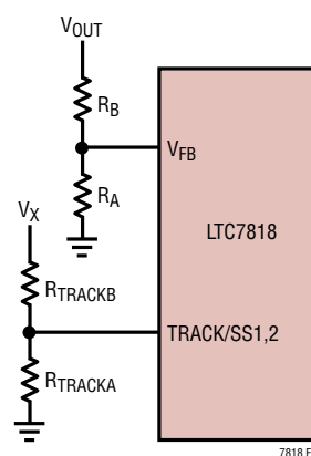
Figure 8. Using the TRACK/SS Pin for Tracking
