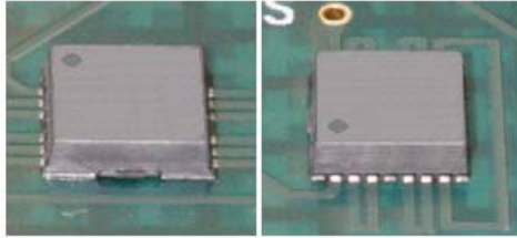
Figure 9. Solder pads, component leads and the solder joints are located under the component itself.
