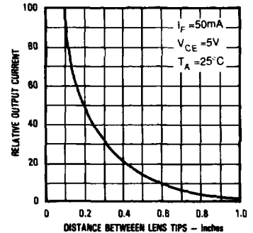
Coupling Characteristics of OP123 and OP600
