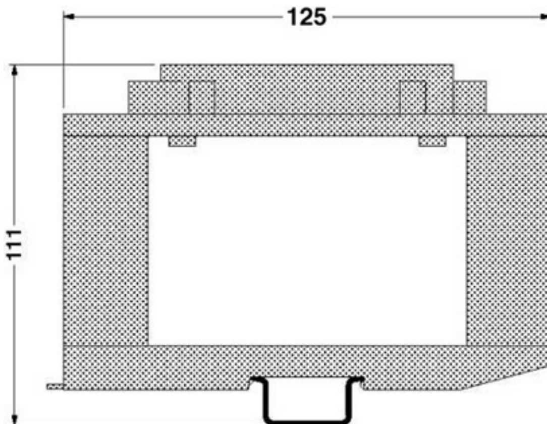
Dimensioned drawing
