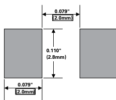
Recommended Soldering Pad Outline
