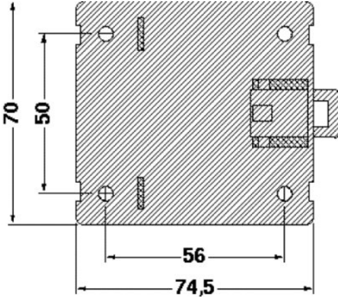
Dimensional drawing
