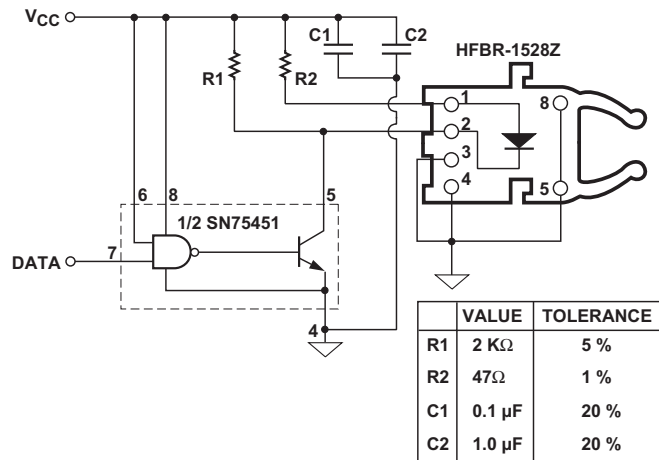
Figure 6. Recommended transmitter drive circuit ( I_{r,on} = 60 mA nominal at T_A = 25^\circ\text{C} )
