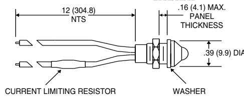
PH31 Dimensions
