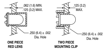
PH25 Mounting
