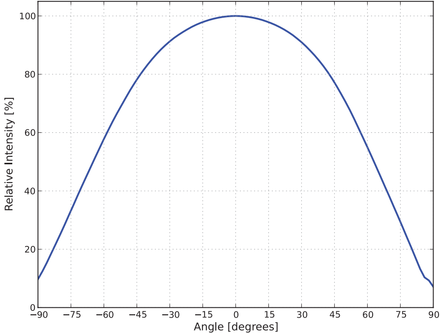
Figure 4: Typical radiation pattern for LUXEON TX at 700mA, T_j=85^{\circ}\text{C} .
