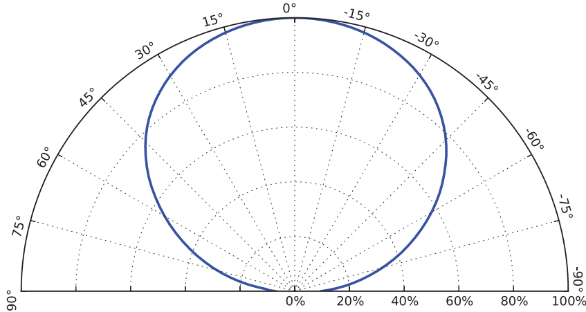
Figure 5: Typical polar radiation pattern for LUXEON TX at 700mA, T_j=85^{\circ}\text{C} .
