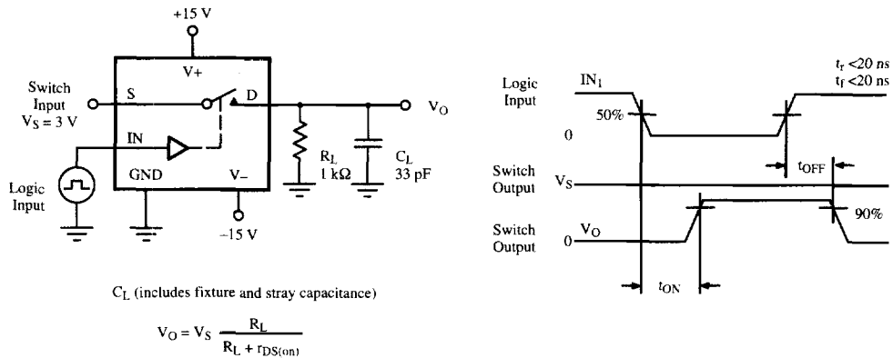
Figure 2. Switching Time
