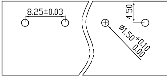
PCB LAYOUT
