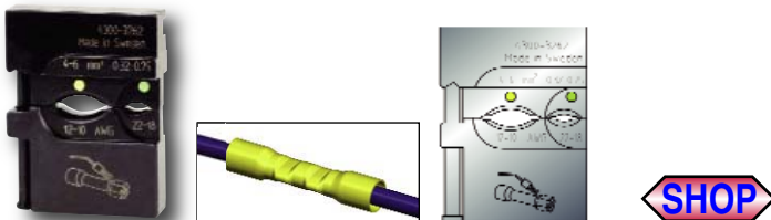
431 62 PortaCrimp Die set for heat shrink connectors: 4-6mm 2 yellow & 0.32-0.75mm 2 green.
