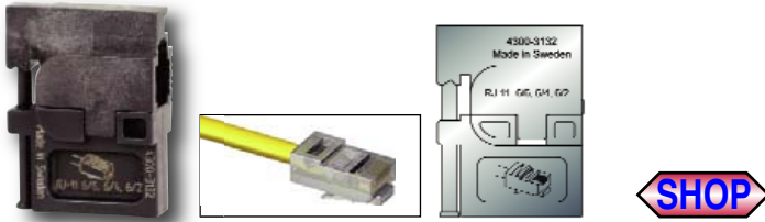
431 32 PortaCrimp Datacom/Telecom Modular Plug Die set for 6-position 6-contact (RJ11).
