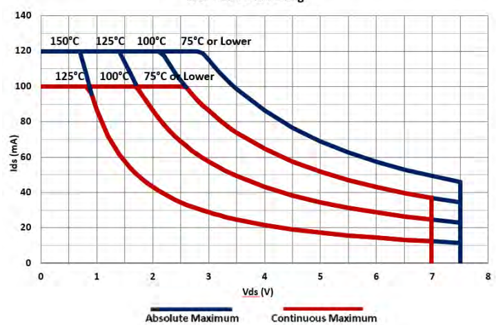
Thermal Safe Operating Limits vs Backside Temperature MwT-3F 70 & 73 Pkg
